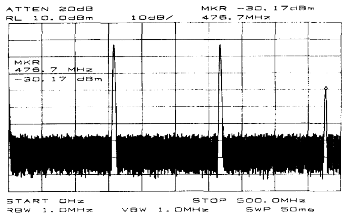
Fig. 8 Regenerative divide-by-five operation
