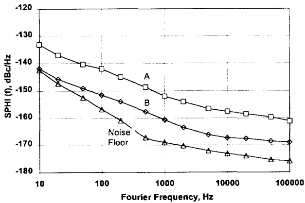
Fig. 6 Phase noise measurements of the divide-by-four circuit
