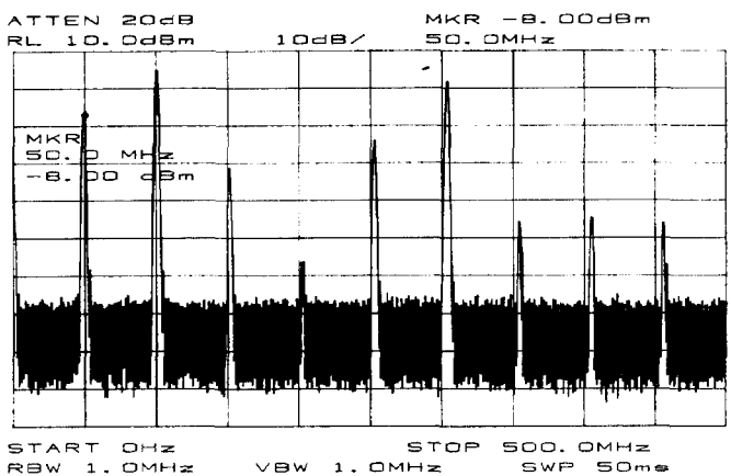
Fig. 9 Regenerative divide-by-nine operation
